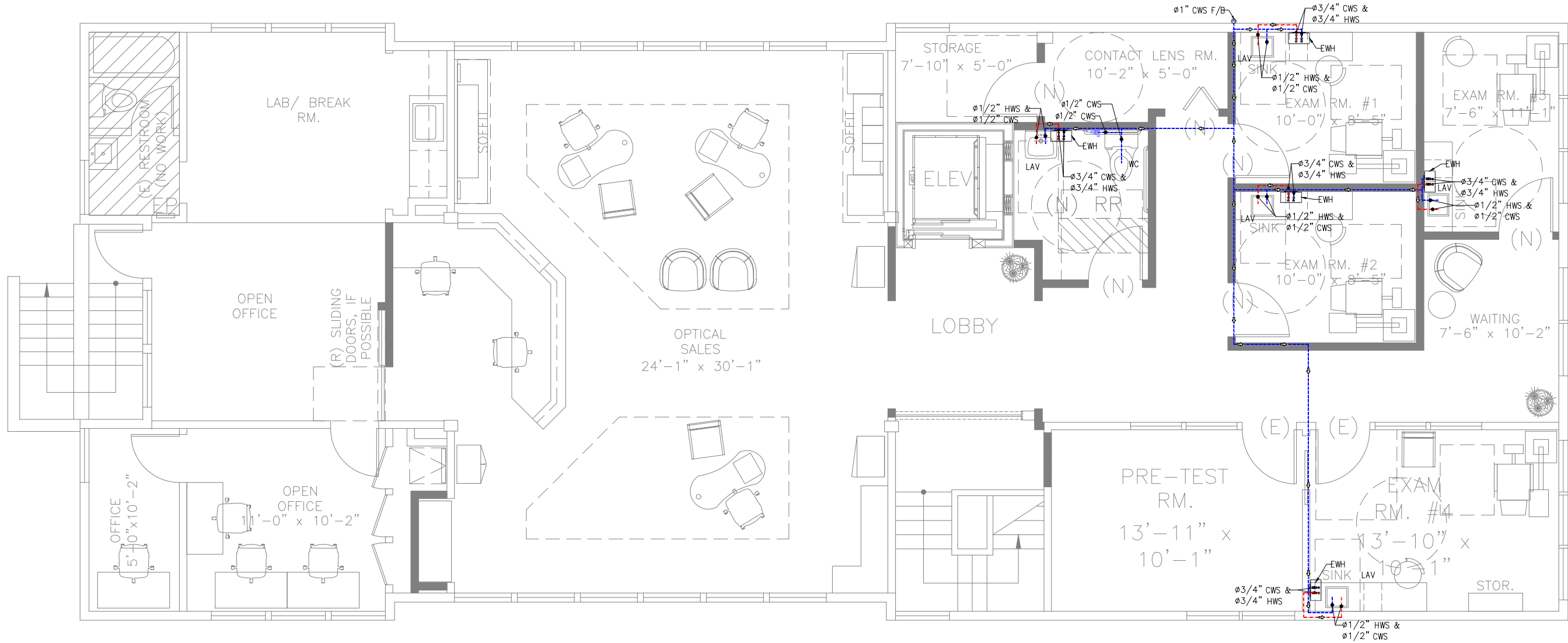
PL 05 SCALE SECOND FLOOR WATER SUPPLY PLAN 3/16"=1'-0"
