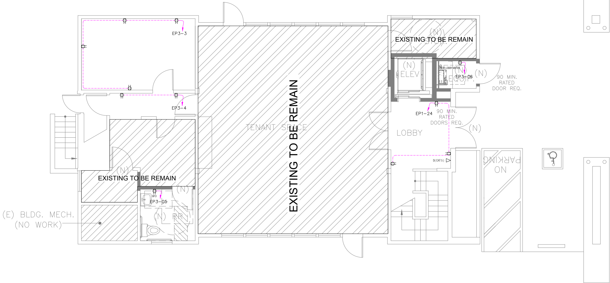
EL 04 FIRST FLOOR POWER PLAN SCALE 1/8"=1'-0"
