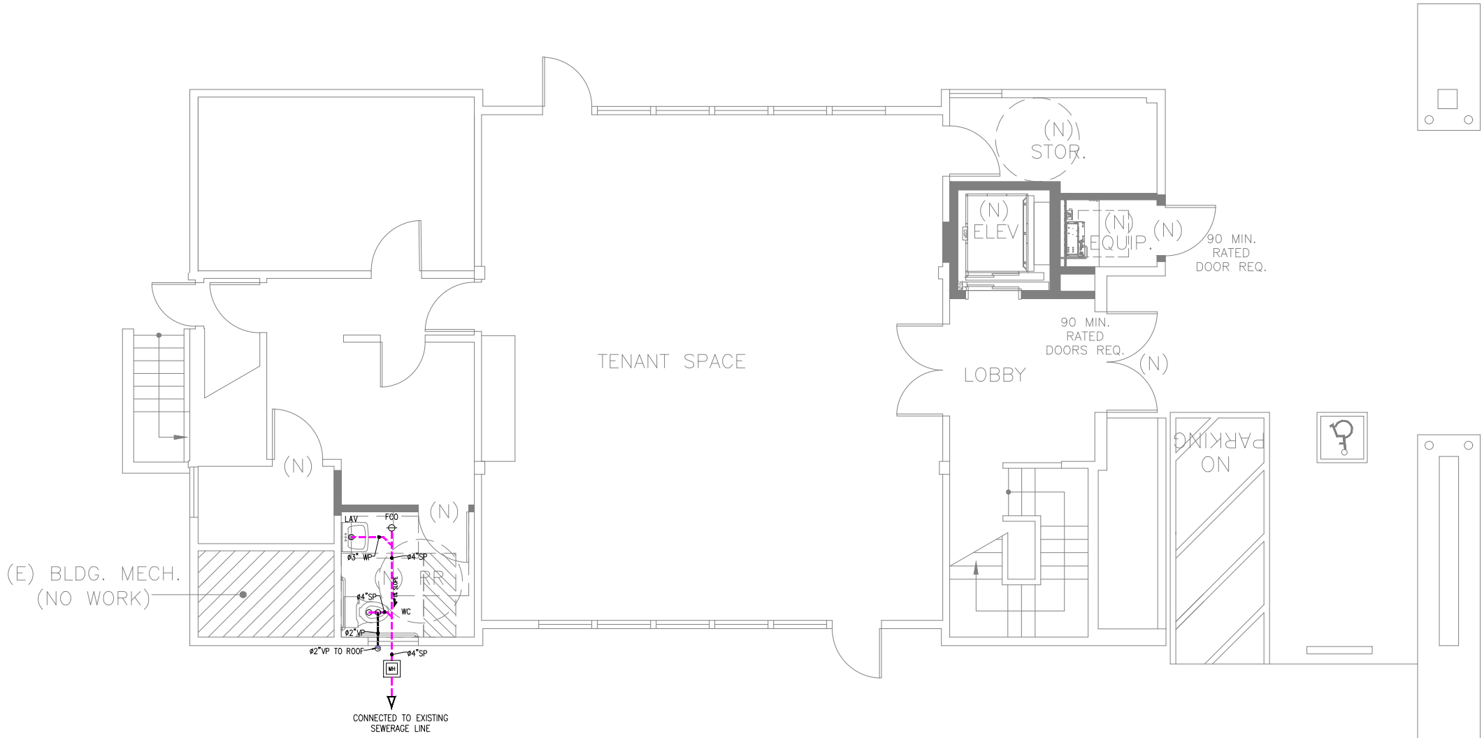
PL 02 FIRST FLOOR DRAINAGE PLAN SCALE 1/8"=1'-0"
